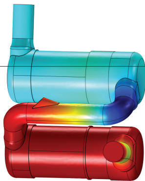
The sound pressure distribution across the inner surface of a silencer at a single frequency (f = 100 Hz).
